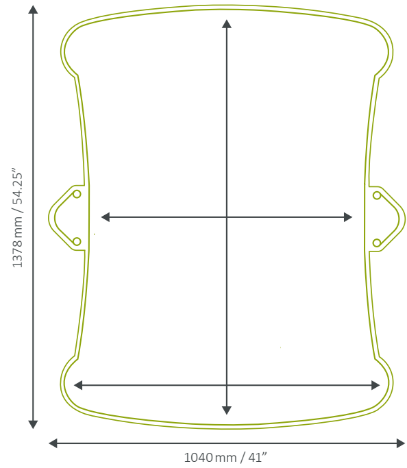
Trio+ Footprint
