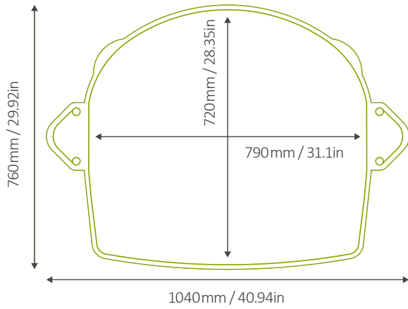
Duo+ Footprint
